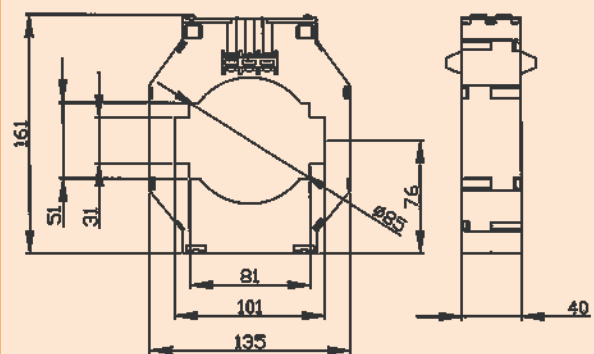
FOX100.3 DIMENSIONS
