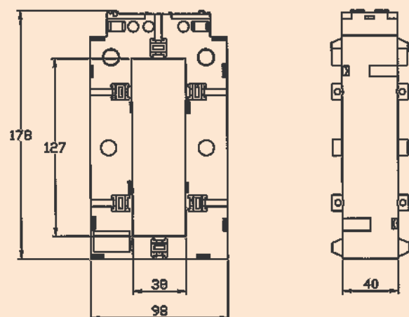
FOX127.38 DIMENSIONS
