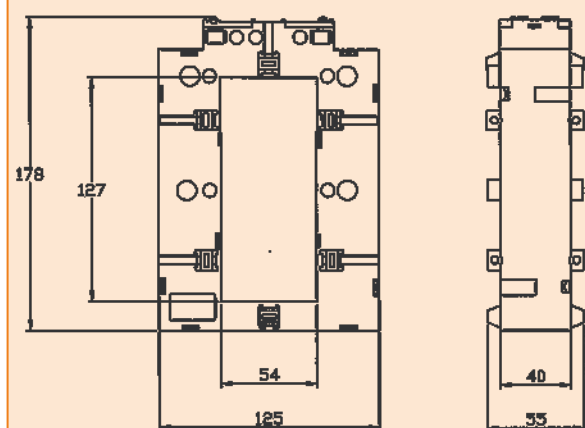
FOX127.54 DIMENSIONS
