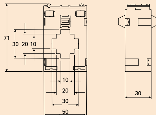
FOX30.1 DIMENSIONS
