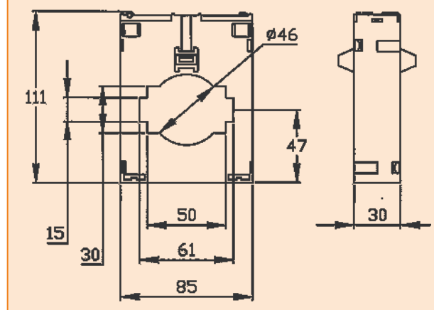
FOX60.15 DIMENSIONS
