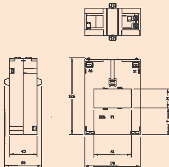
FOX60.3 DIMENSIONS
