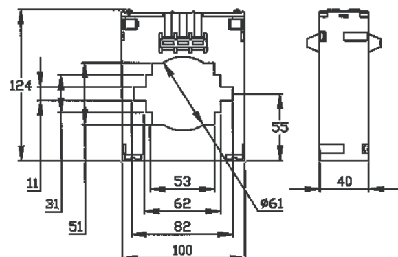
FOX80.1 DIMENSIONS
